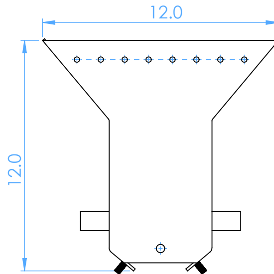
Model DI-2 12in x 12in
