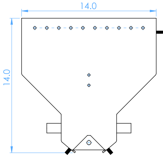
Model DE 14in x 14in
